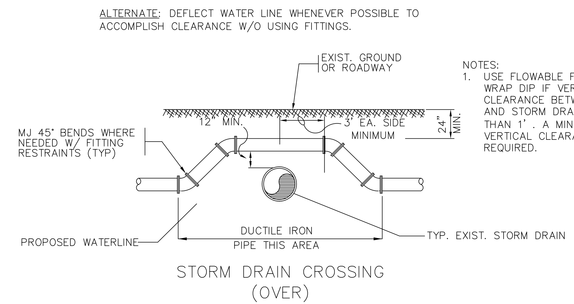
STORM DRAIN CROSSING (UNDER)
